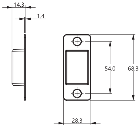
CSM72-P150 STANDARD STRIKE BOX
