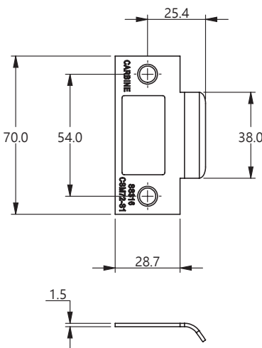
CSM72-S1-SS 25MM STRIKE PLATE
