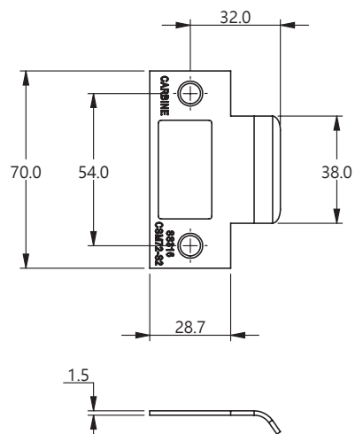
CSM72-S2-SS 32MM STRIKE PLATE
