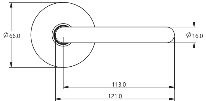
CRF136-L7-SS - EXTERNAL SIDE
