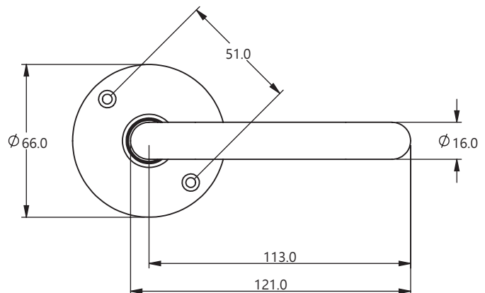
CRF136-L7-SS - INTERNAL SIDE
